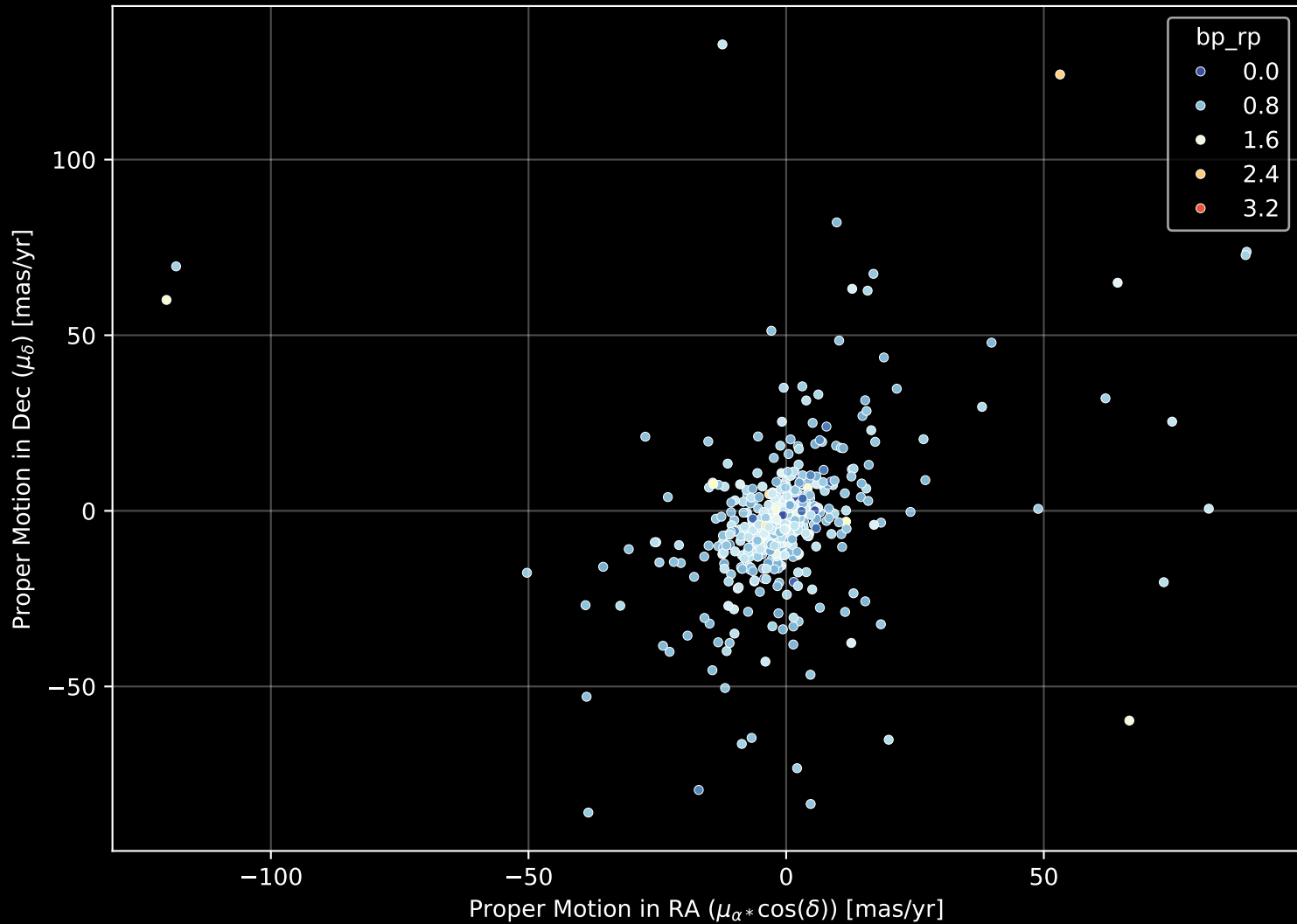
APOGEE DR17 Field: [K05_080+14] Proper Motion Diagram (n= 573)
