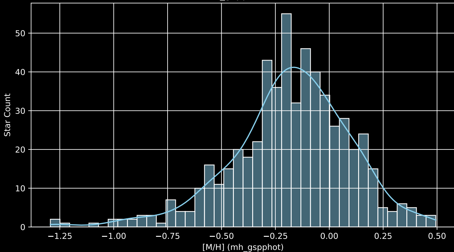
APOGEE DR17 Field: [K05_080+14 [M/H] (mh_gspphot) (n= 569)
