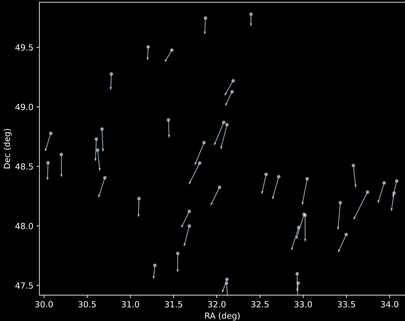
APOGEE DR17 Cluster 21 Proper Motion Vectors (n=42)
