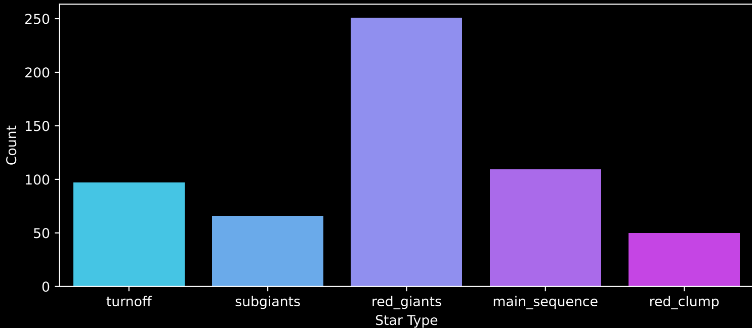
APOGEE DR17 Field: [K05_080+14] Count plot of Star Type
