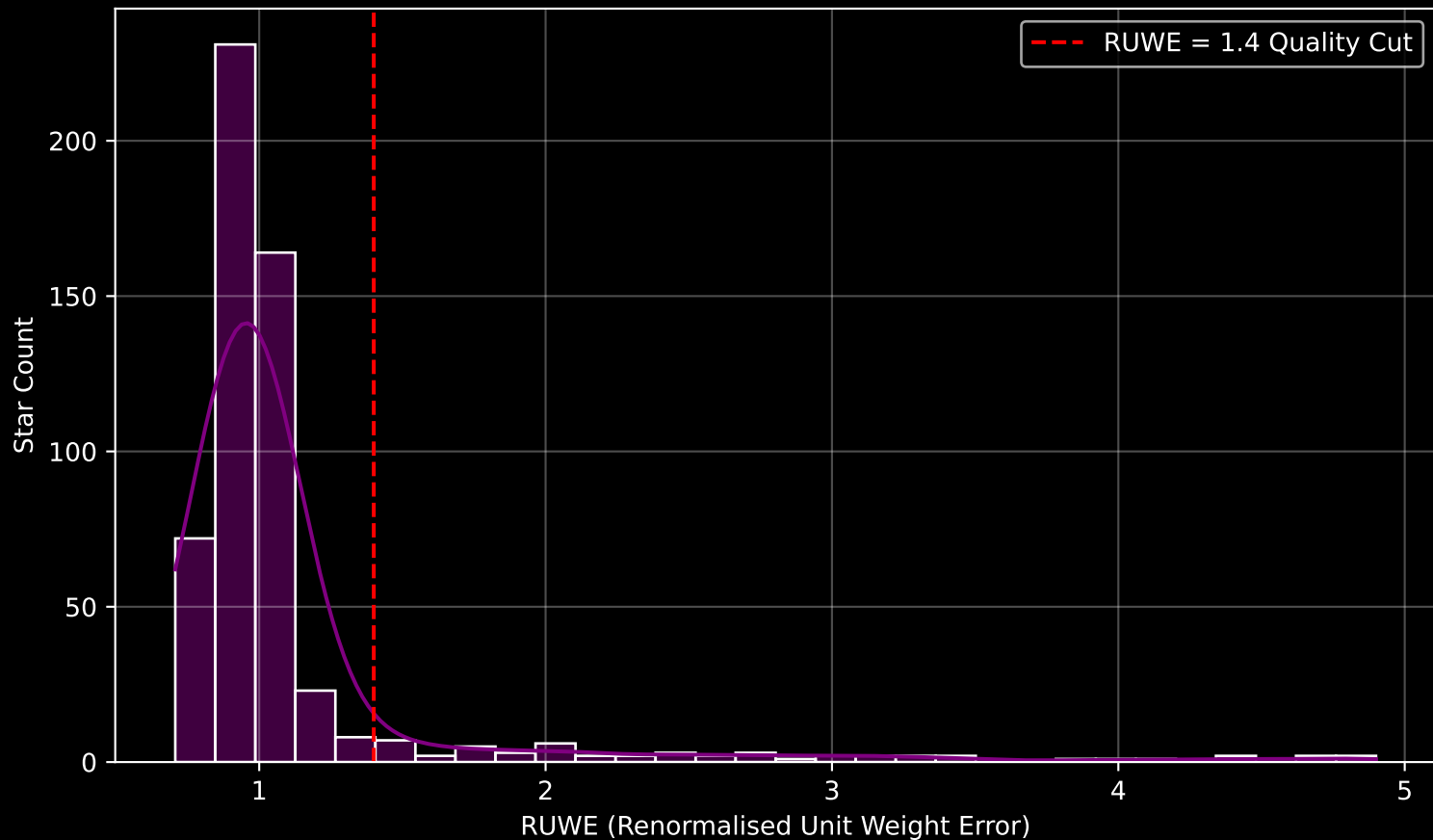
GAPOGEE DR17 Field [K05_080+14] RUWE Distribution (n= 551)
