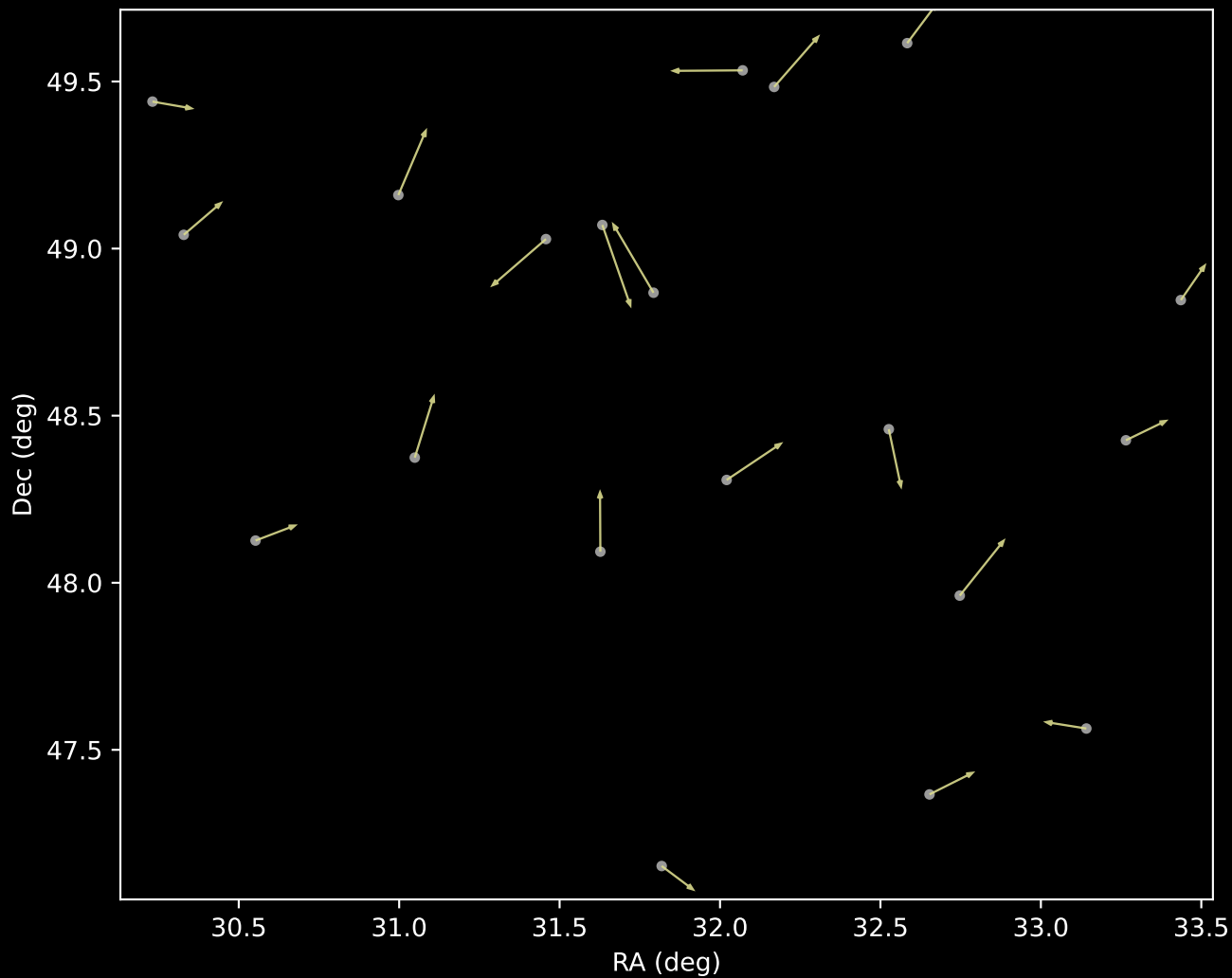
APOGEE DR17 Cluster 17 Proper Motion Vectors (n=20)
