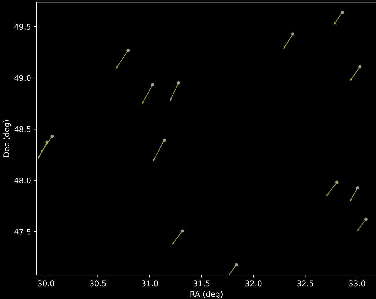
APOGEE DR17 Cluster 16 Proper Motion Vectors (n=14)
