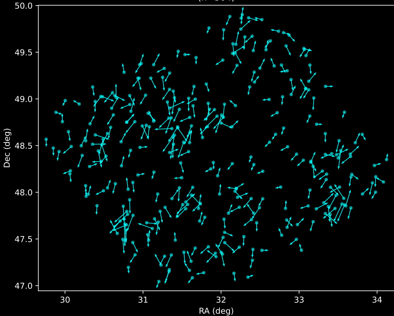
APOGEE DR17 Noise Stream Proper Motion Vectors (n=304)
