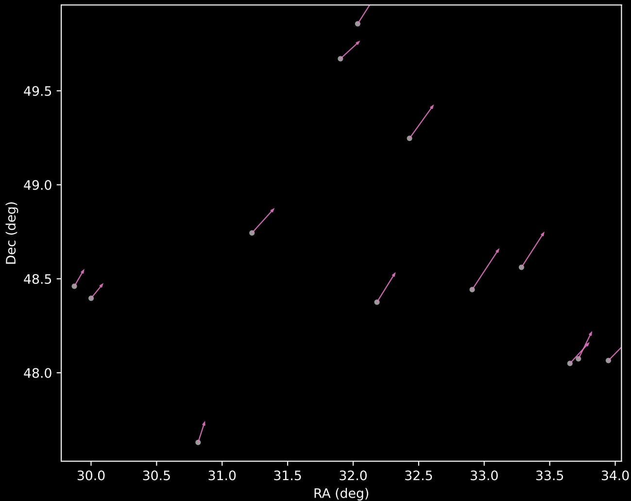
APOGEE DR17 Cluster 12 Proper Motion Vectors (n=13)
