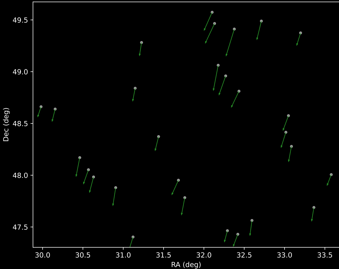
APOGEE DR17 Cluster 24 Proper Motion Vectors (n=28)
