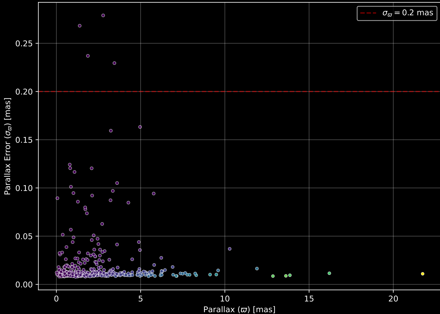
APOGEE DR17 Field: [K05_080+14] Parallax Quality (n= 573)
